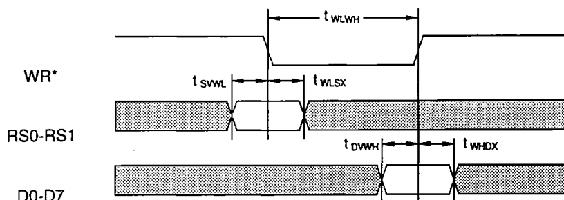
Basic Write Cycle Timing
