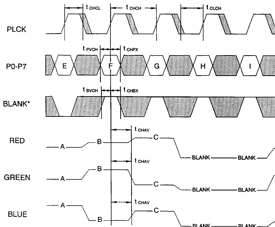
Detailed Timing Specifications - Pseudo Color, Mode 0
