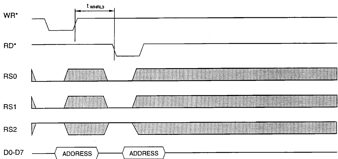
Write and Read back PLL Address Register (Write Mode)
