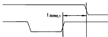
Read from Pixel or Pixel Address Register (Read or Write) followed by Write
