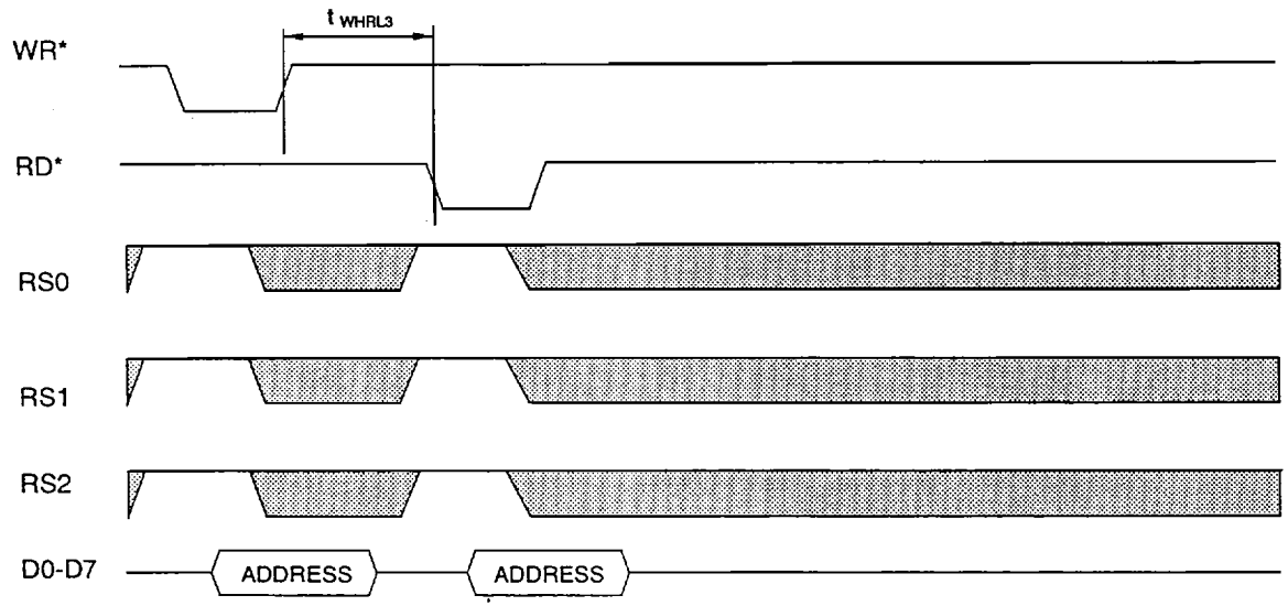
Write and Read back PLL Address Register (Read Mode)
