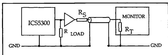
Figure 2 - Buffered Signal
