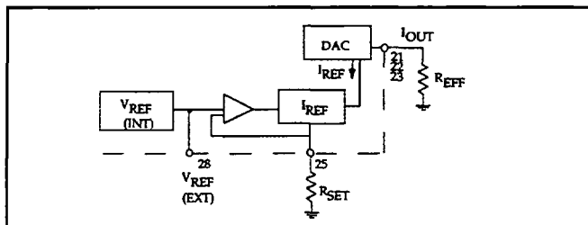
Figure 4 - DAC Set up
