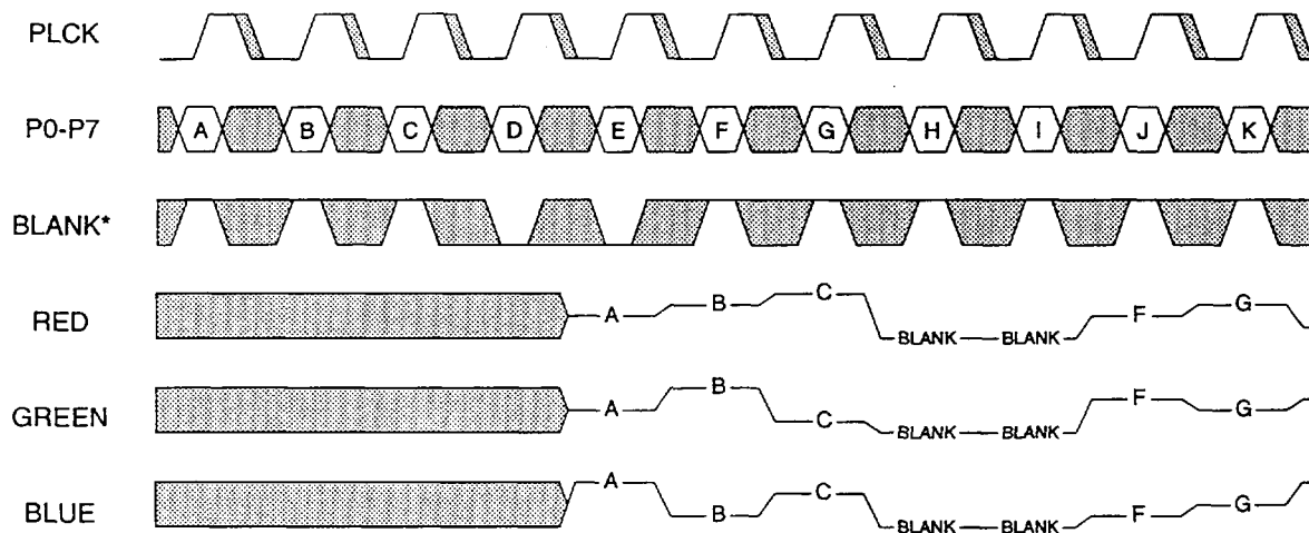
System Timing - Pseudo Color, Mode 0
