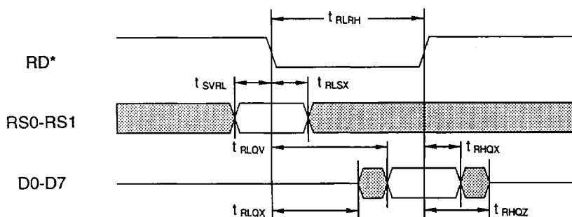
Basic Read Cycle Timing
