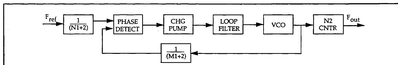
Figure 3 - PLL Clock Synthesizer Block Diagram
