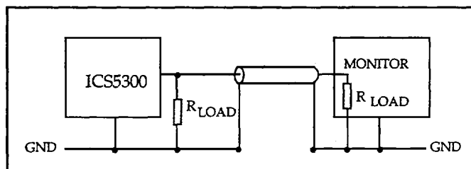
Figure 1 - Double Termination
