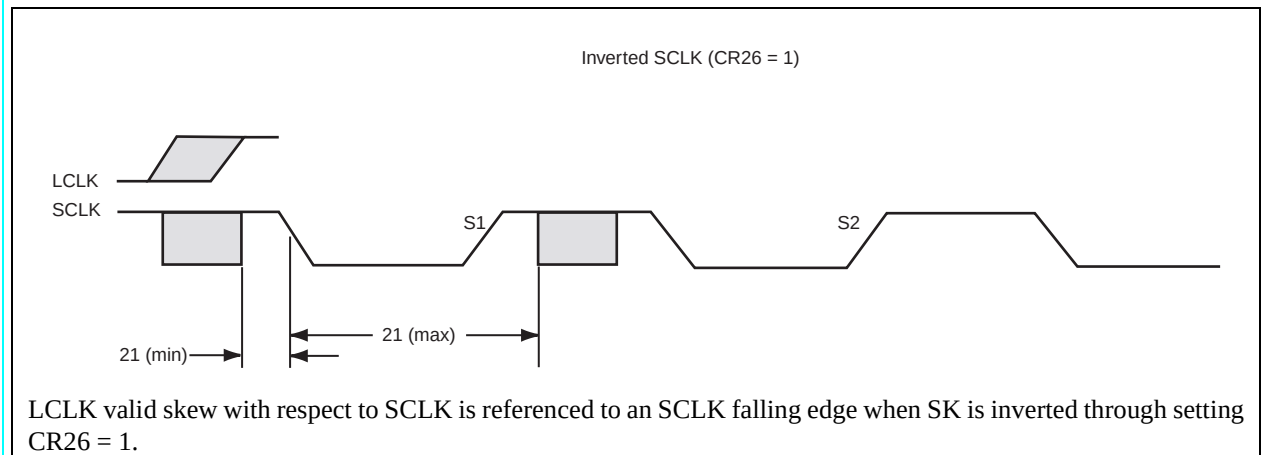
Figure 17. SCLK to LCLK Timing (Non-1:1)
