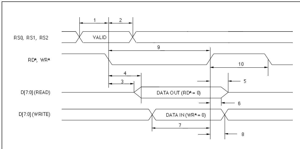
Figure 15. MPU Read/Write Timing.
